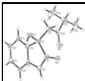
Fig. 1. An ORTEP-3 drawing of compound I, with the atom-numbering scheme and 30% probability displacement ellipsoids.
