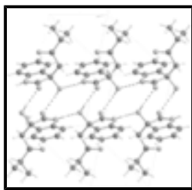
Fig. 2. Packing diagram of the title compound. Dashed lines indicate hydrogen bonds.
